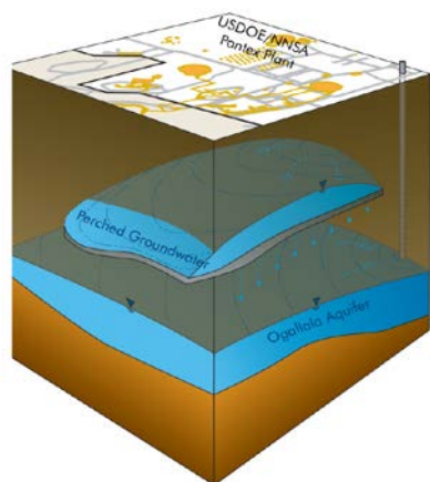
Groundwater Beneath Pantex
