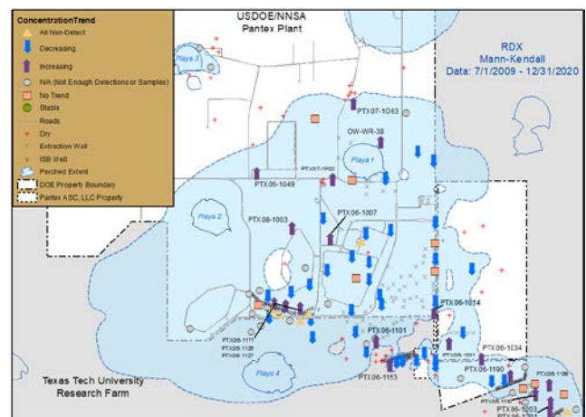
2020 Evaluation of RDX concentration trends based on monitoring data collected at perched groundwater wells
