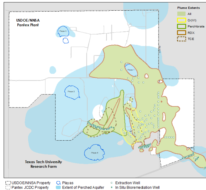
Extent of Perched Groundwater and Plumes (2020)
